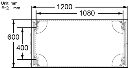
Bottom view of the precision PDF / 精密配电柜底部视图
