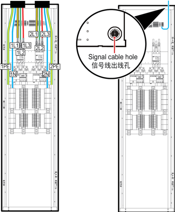
Front view of the precision PDF / 精密配电柜前视图 Front view of the precision PDF / 精密配电柜前视图
