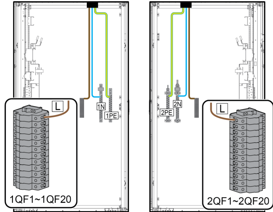
Left view of the precision PDF / 精密配电柜左侧视图
