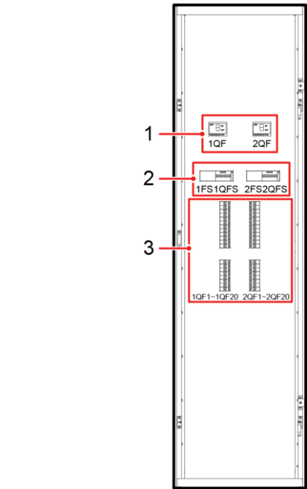
Front view of the precision PDF / 精密配电柜前视图
